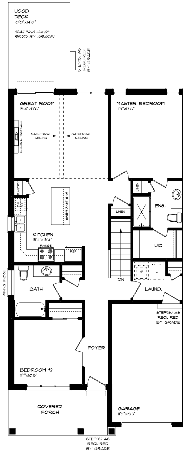
HALLWOOD (PREMIUM SPECS) LOT 45A (#6) HEMLOCK CRESCENT MAIN FLOOR PLAN 9' MAIN FLOOR CEILING APPROX. 1,225 SQ. FT.
