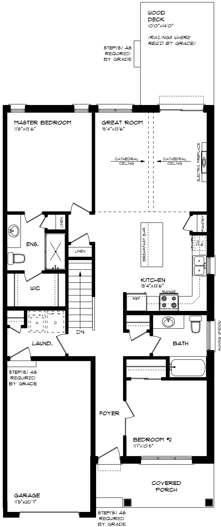
HALLWOOD (PREMIUM SPECS) LOT 46B (#4) HEMLOCK CRESCENT MAIN FLOOR PLAN 9' MAIN FLOOR CEILING APPROX. 1,225 SQ. FT.
