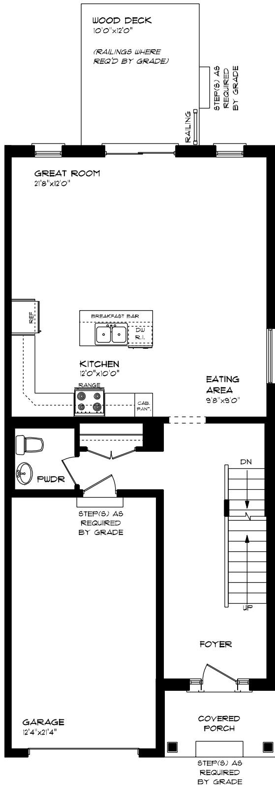
TIFTON (ESSENTIAL SPECS) LOT 5F (#93) WILLOW DR. MAIN FLOOR PLAN 8' MAIN FLOOR CEILING APPROX. 852 SQ. FT.
